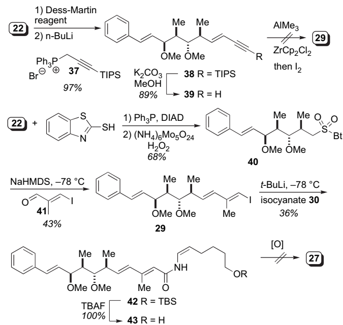
Scheme 8. Synthesis of iodide 29 and anion coupling.
