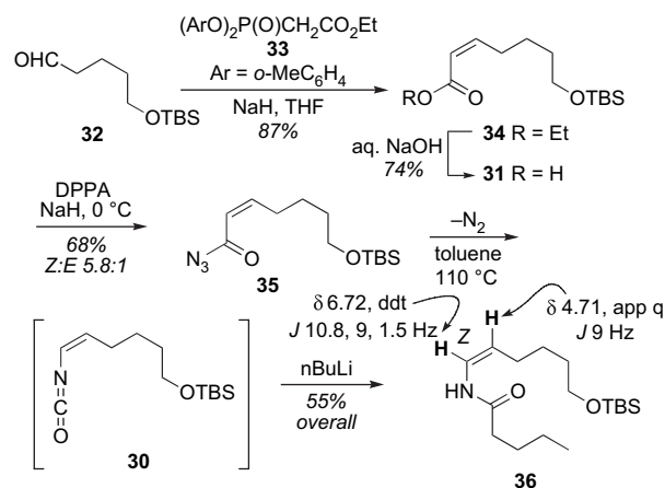
Scheme 7. Synthesis of the Z-vinylisocyanate 30 .
