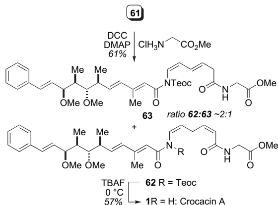
Scheme 15. Alternative synthesis of crocacin A (1).
