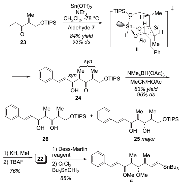
Scheme 4. Synthesis of vinyl stannane 5 .
