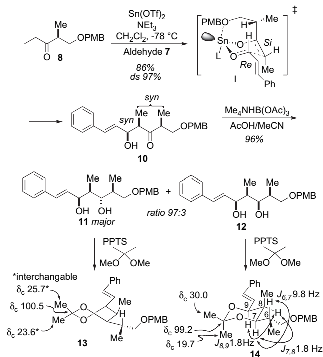
Scheme 2. Synthesis of the stereotetrad 11 .
