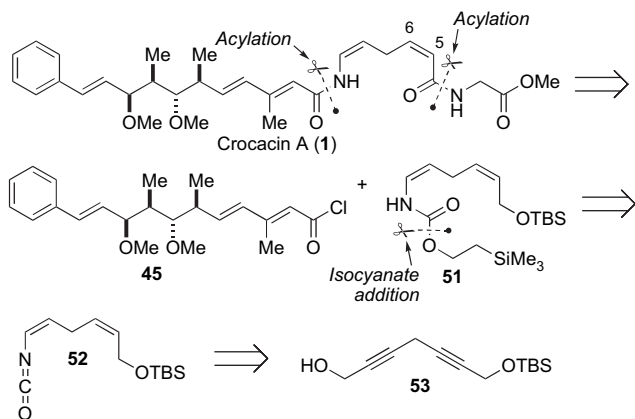
Scheme 12. Retrosynthetic analysis of crocacin A ( 1 ).
