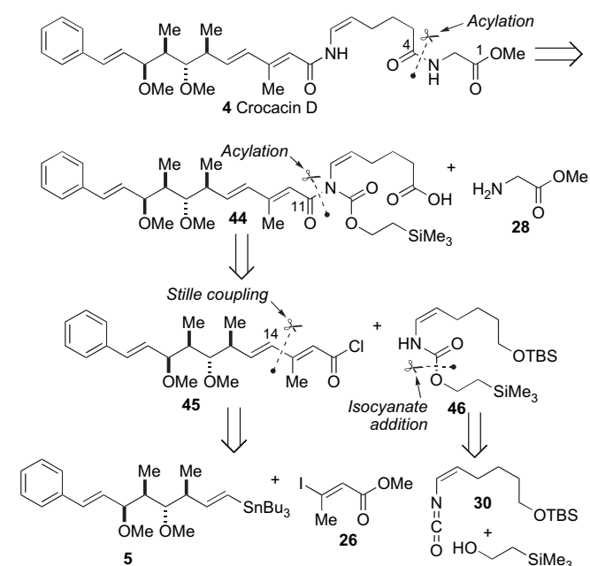
Scheme 9. Alternative approach to crocin D ( 4 ).
