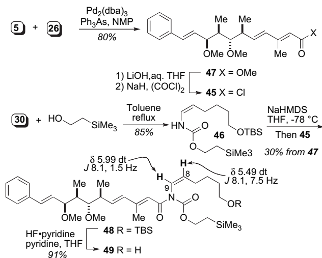
Scheme 10. Acylation of enecarbamate 46 with acid chloride 45 .
