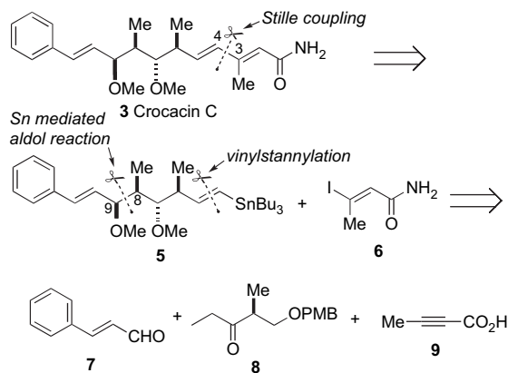
Scheme 1. Retrosynthetic analysis of crocacin C ( 3 ).
