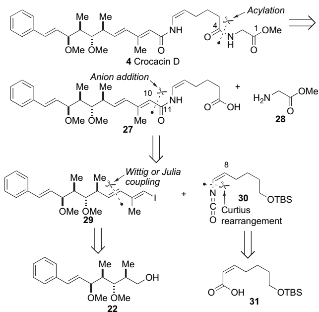
Scheme 6. Initial retrosynthetic analysis of crocacin D (4).
