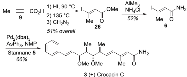
Scheme 5. Total synthesis of (+)-crocacin C (3).
