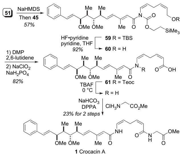
Scheme 14. Total synthesis of crocacin A (1).
