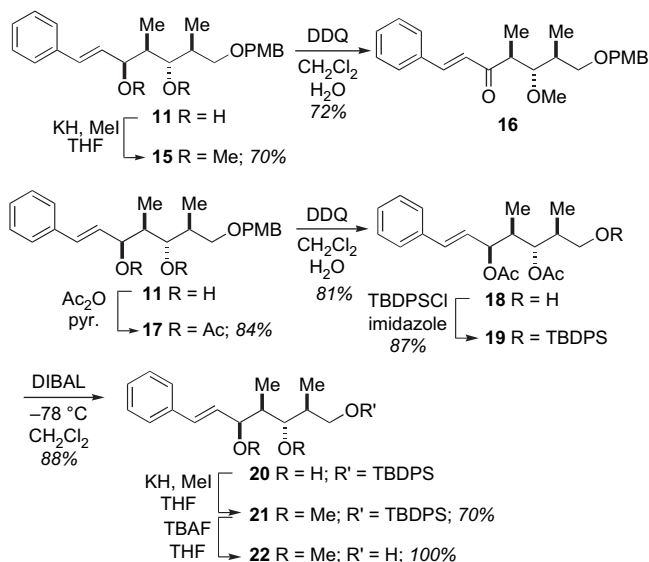
Scheme 3. Synthesis of intermediate alcohol 22 .
