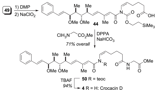
Scheme 11. Total synthesis of crocacin D ( 4 ).
