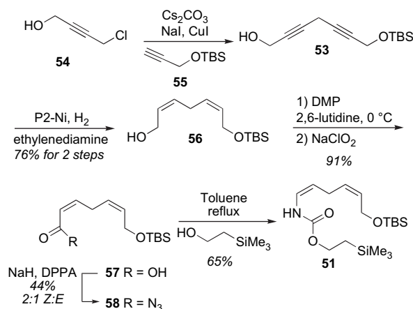
Scheme 13. Synthesis of dienecarbamate 51 .
