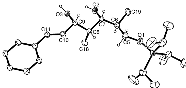
Figure 1. X-ray structure of diol 26 (some H atoms omitted for clarity).
