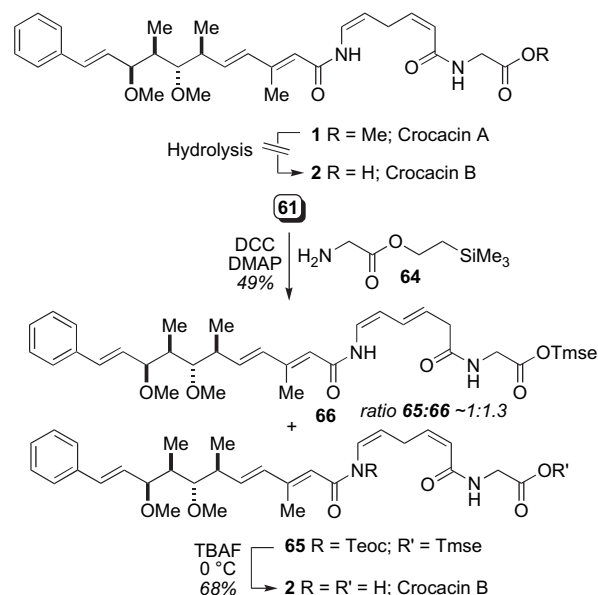
Scheme 16. Total synthesis of crocacin B (2).
